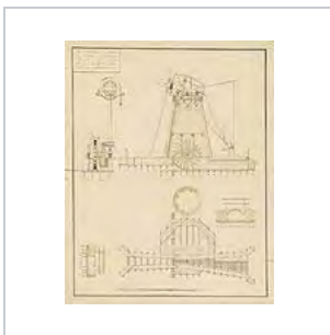
Technical drawing of a 1793 Dutch tower mill for land drainage
