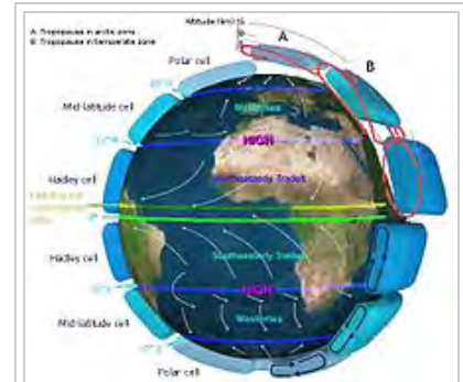
Winds are part of Earth's atmospheric circulation.
