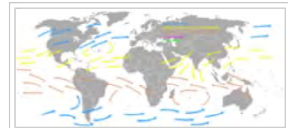
The westerlies and trade winds
