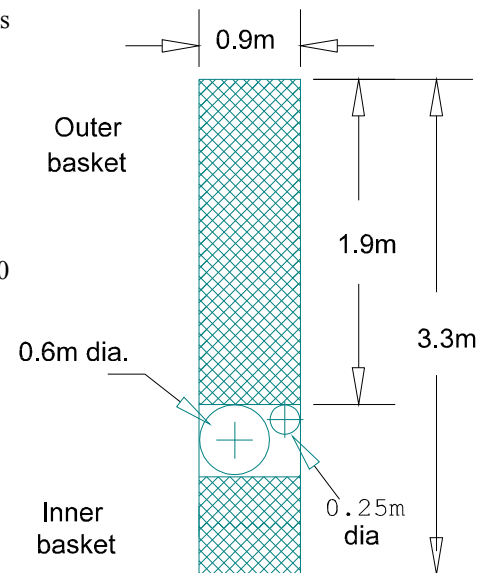
Cutting plan for wire mesh
