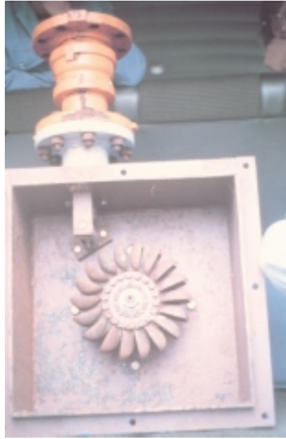
Even seasonal streams will supply power in the winter from units like this pelton wheel.
