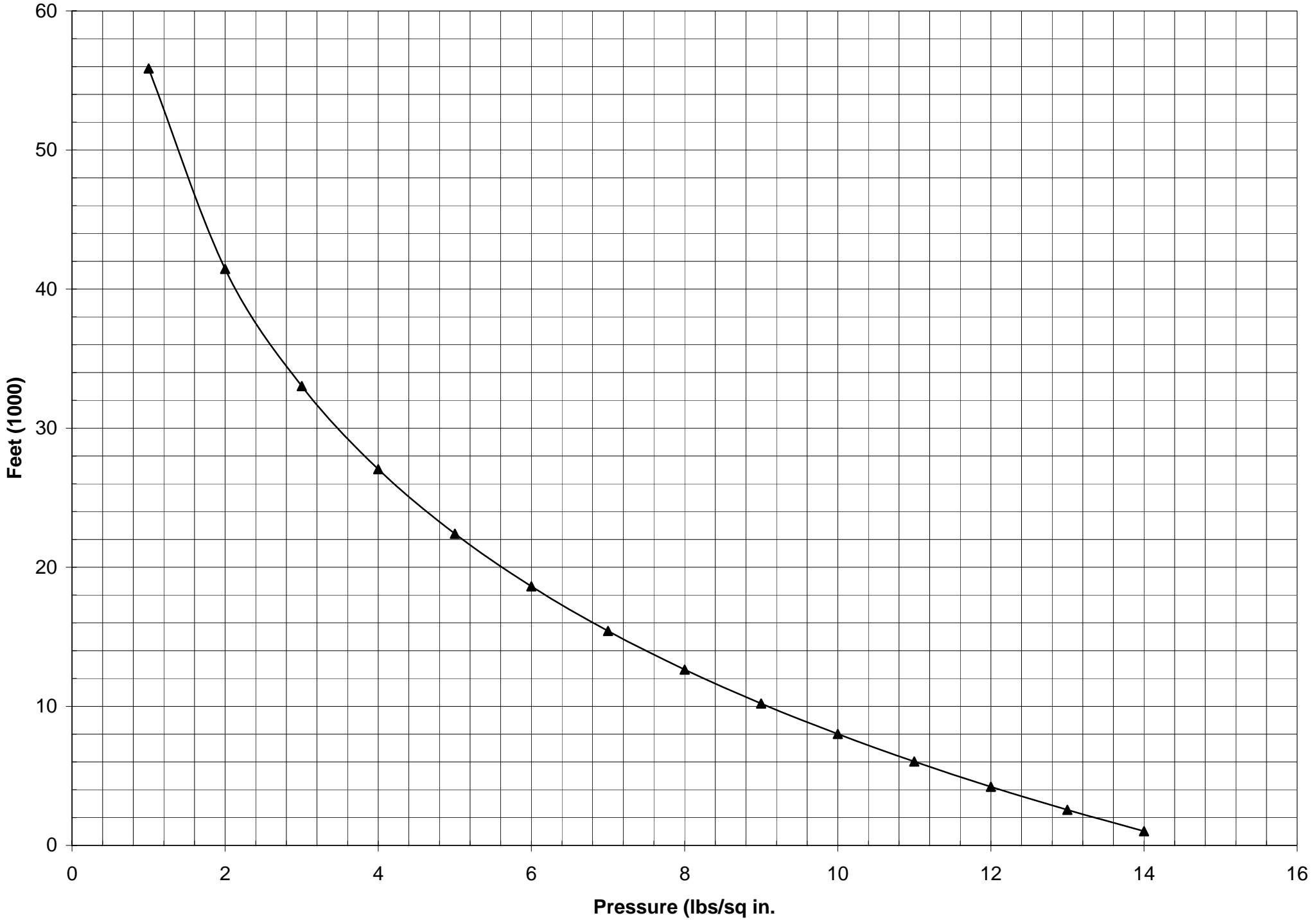
Atmospheric Pressure versus Height
