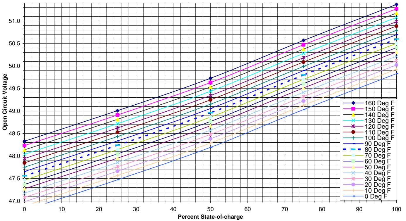
48 Volt Lead-Acid Deep Cell State-of-Charge versus Voltage & Temperature
