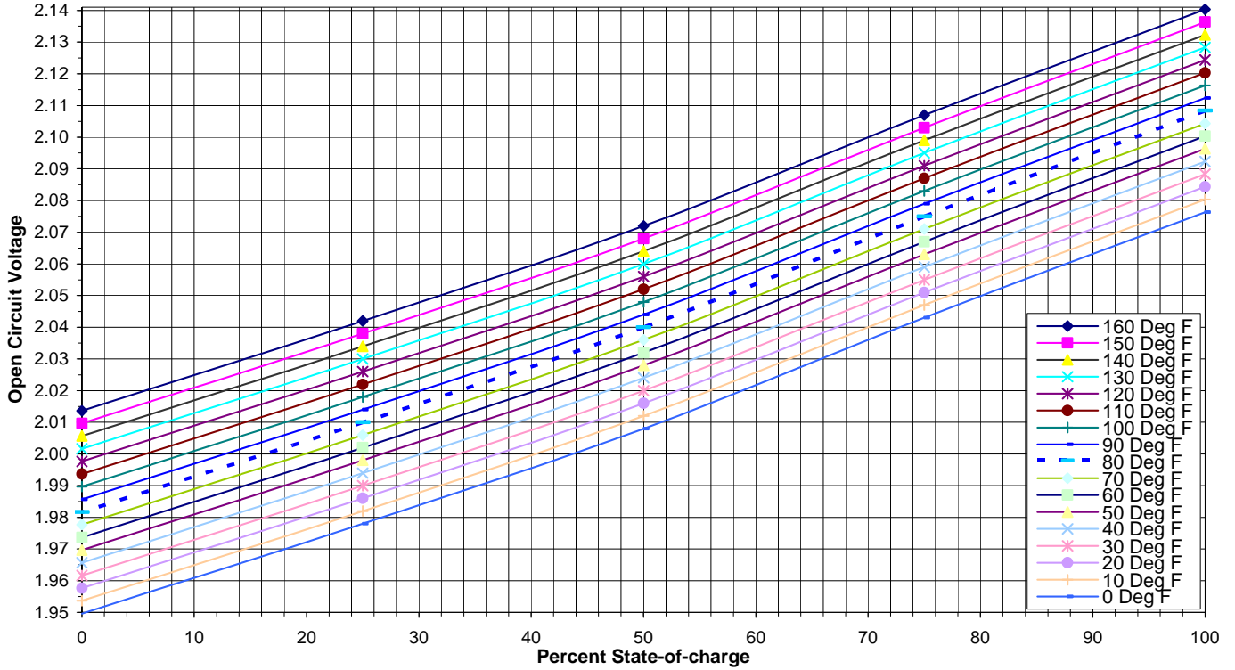
One 2 Volt Lead-Acid Cell State-of-Charge versus Voltage & Temperature
